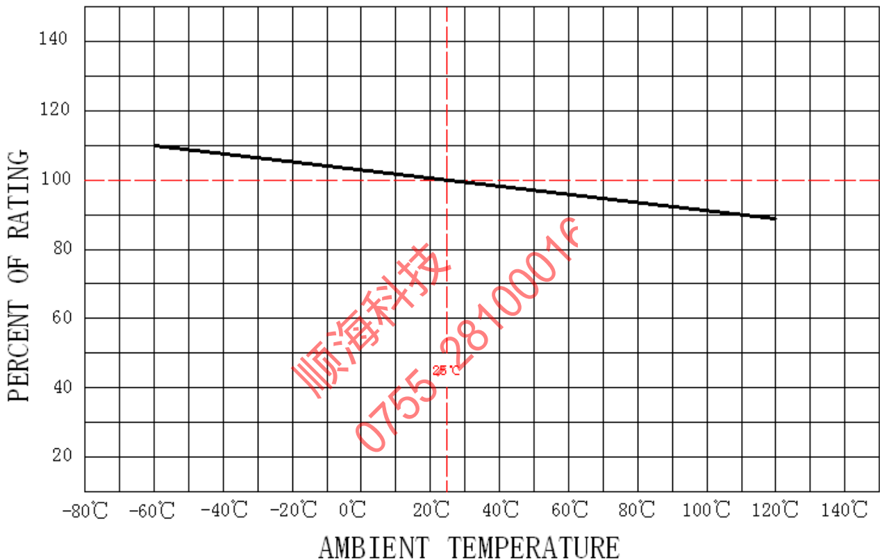
Temperature-Current curve:
